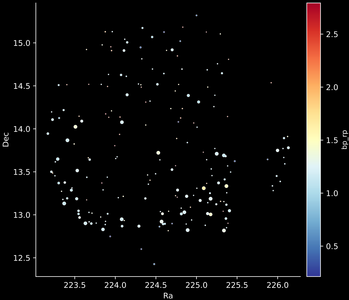
APOGEE DR17 Field: [K2_C18_210+25_btx] Stars: 203
