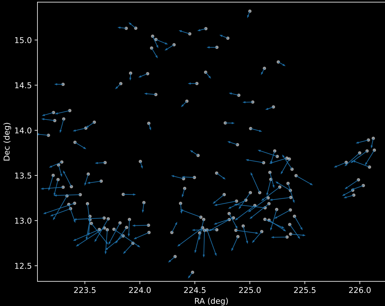
APOGEE DR17 Cluster 0 Proper Motion Vectors (n=134)
