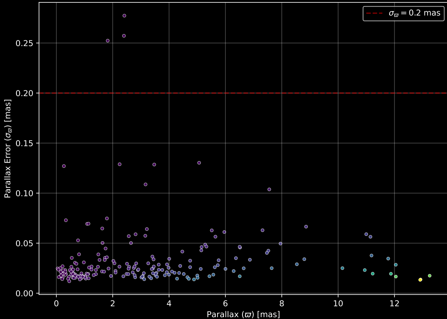
APOGEE DR17 Field: [K2_C18_210+25_btx] Parallax Quality (n= 203)
