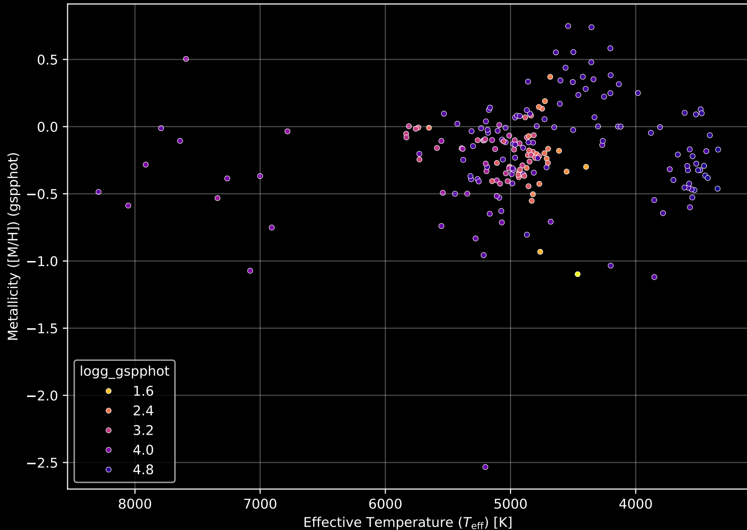
APOGEE DR17 Field: [K2_C18_210+25_btx] Stellar Population Parameters (n= 203)
