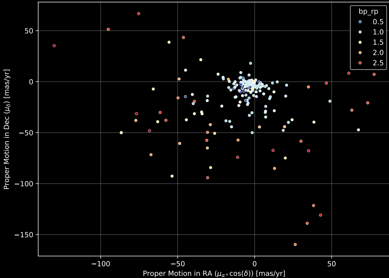
APOGEE DR17 Field: [K2_C18_210+25_btx] Proper Motion Diagram (n= 203)
