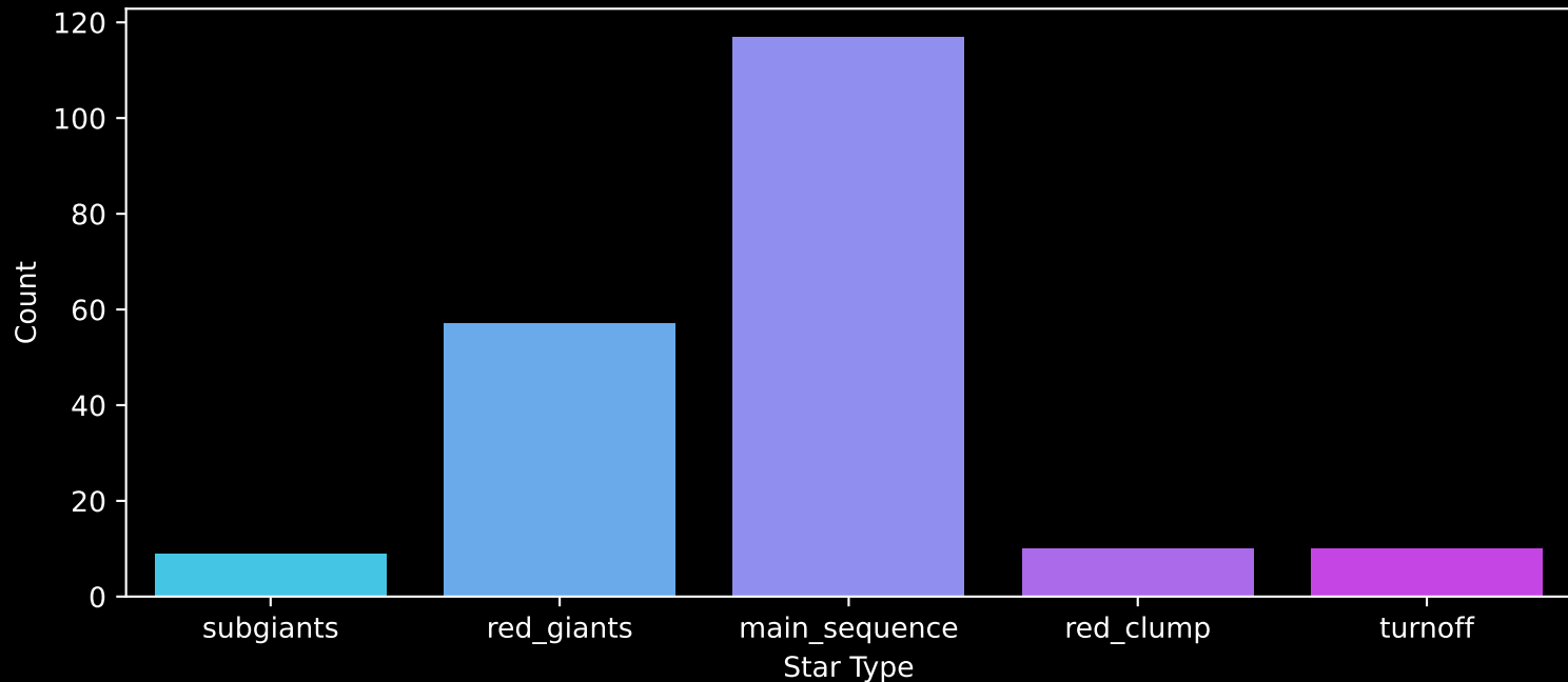
APOGEE DR17 Field: [K2_C18_210+25_btx] Count plot of Star Type
