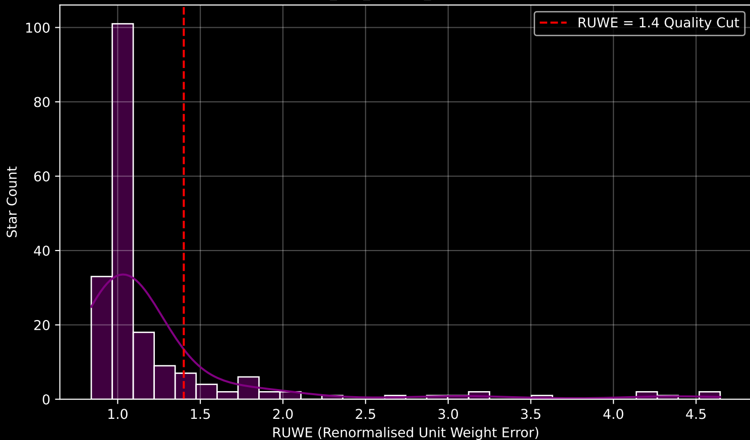
GAPOGEE DR17 Field [K2_C18_210+25_btx] RUWE Distribution (n= 196)
