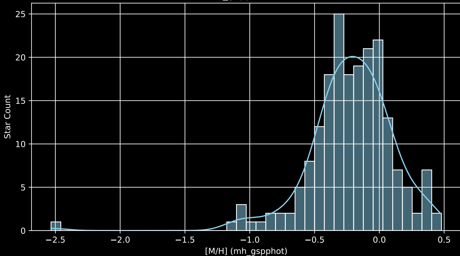
APOGEE DR17 Field: [K2_C18_210+25_btx [M/H] (mh_gspphot) (n= 197)
